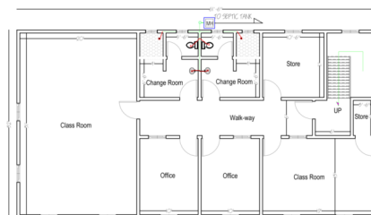
Proposed Upper Floor Plan
